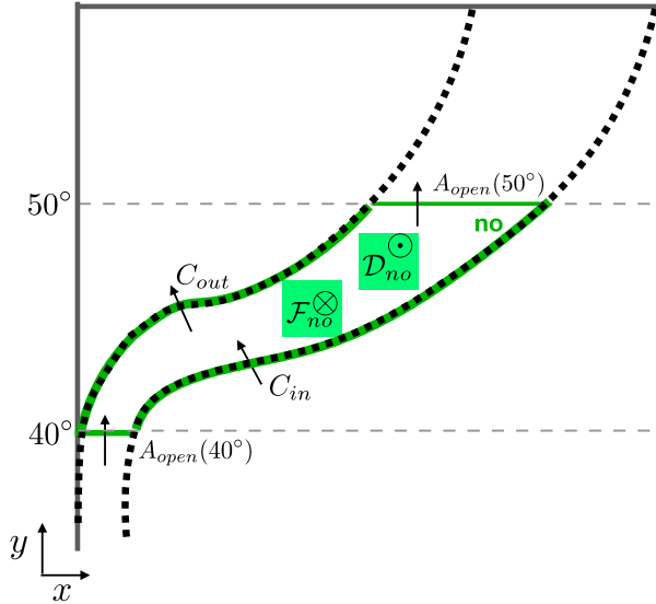
FIG. 7. Schematic of salt transport into the region of open streamlines between 40^\circ and 50^\circ . The solid gray lines represent the boundaries of the domain, and the black dotted lines represent the easternmost and westernmost open streamlines; C_{in} is the horizontal cross-streamline salt transport above the isopycnal b_m into the region of open streamlines (the area bounded by green lines) from the south, \mathcal{F}_{no} is the salt transport into the region of open streamlines at the surface, \mathcal{D}_{no} is the diapycnal salt transport across b_m into the region of open streamlines, C_{out} is the horizontal cross-streamline salt transport above the isopycnal b_m out of the region of open streamlines into the north, and A_{open} is the meridional salt transport in the region of open streamlines.
