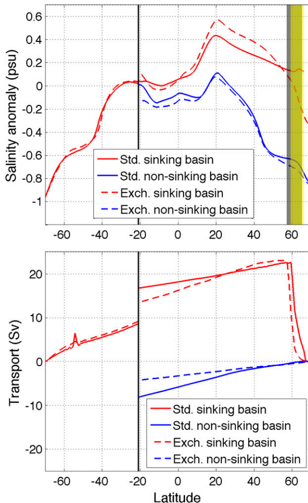
FIG. 5. (top) Salinity anomaly, referenced to 35, depth and zonally averaged above b_m = 0.0066 \text{ m s}^{-2} and across each basin, and (bottom) the residual transport above b_m = 0.0066 \text{ m s}^{-2} in each basin. South of -21^\circ , the zonal integral is taken across all longitudes. The yellow shading indicates the sinking region for the standard geometry, and the gray shading indicates the sinking region for the exchanged geometry. The black vertical line denotes the end of the short continent.
