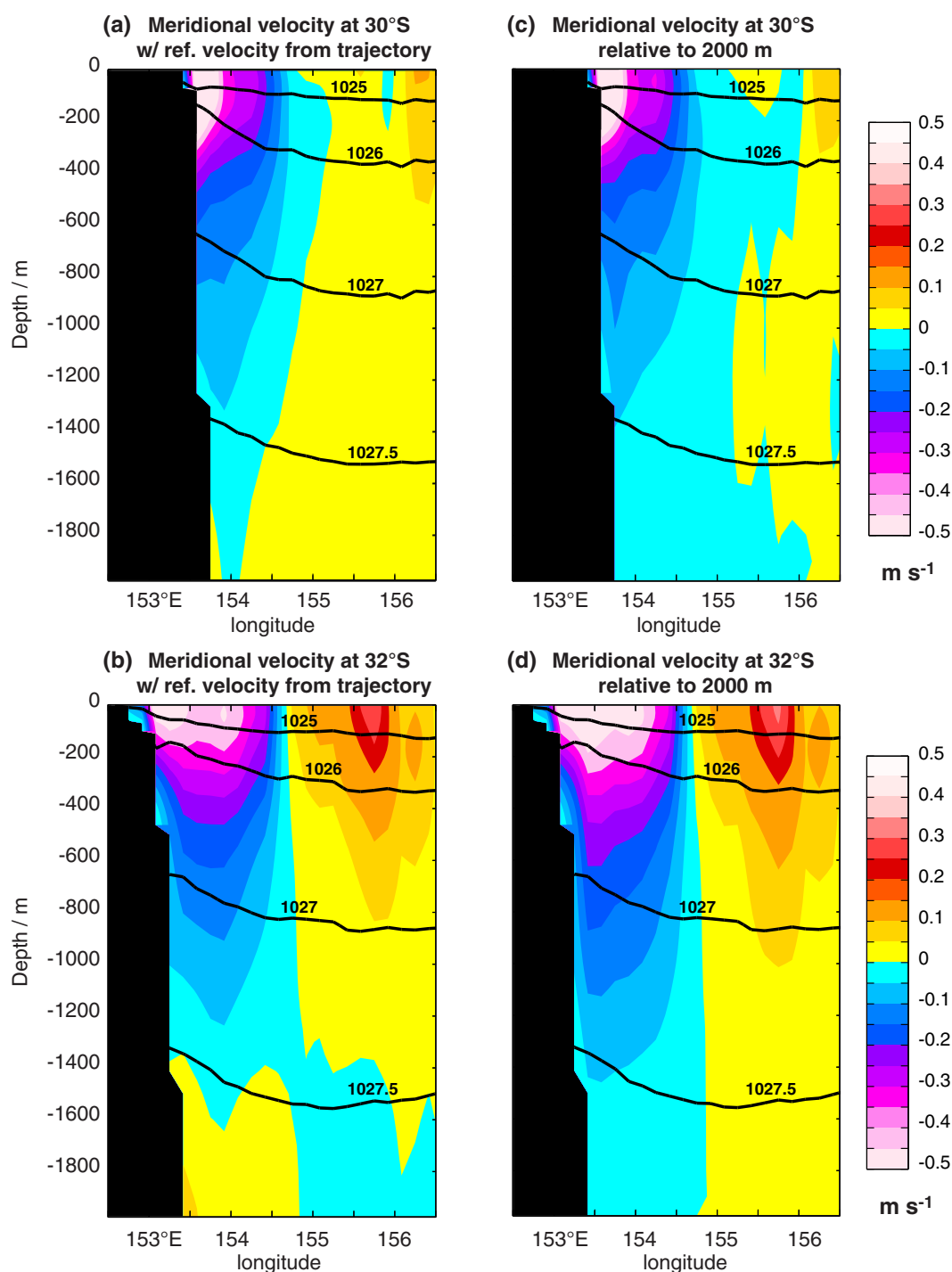
Figure 3. (a and c) Meridional geostrophic velocity in the EAC at 30°S and (b and d) 32°S averaged from 2004 to 2012 with reference velocity using trajectories (Figures 3a and 3b) and relative to 2000 m depth (Figures 3c and 3d). The black lines correspond to 2004–2012 mean potential density contours ( \text{kg m}^{-3} ).
