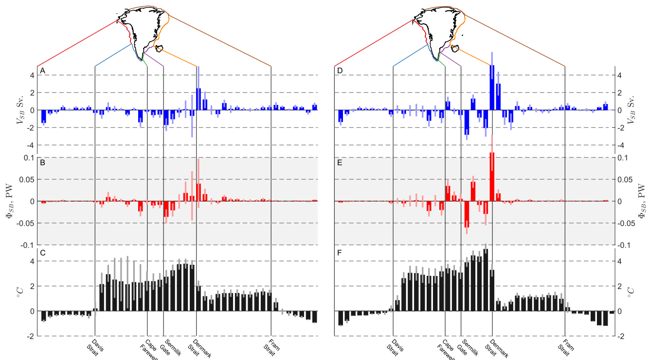
Figure 2. Bar graphs of net volume fluxes (Sv, blue), net heat fluxes (PW, red), and average temperature ( ^{\circ} C, black) for every 100 km section of the transect encircling Greenland for POP (A–C) and HYCOM (D–F). For both volume and heat fluxes, positive values indicate flux onto the continental shelf. Dark bars are the 5-year averages from 2005 to 2009, with light bars representing the 20th and 80th percentile range. In both models, the strongest on-shelf fluxes are near the Denmark Strait. In POP this maximum is associated with strong variability; in HYCOM the heat flux is consistently onto the shelf at this location.
