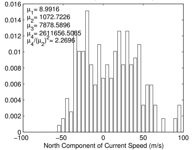
PDF of North Component of Current Speed
