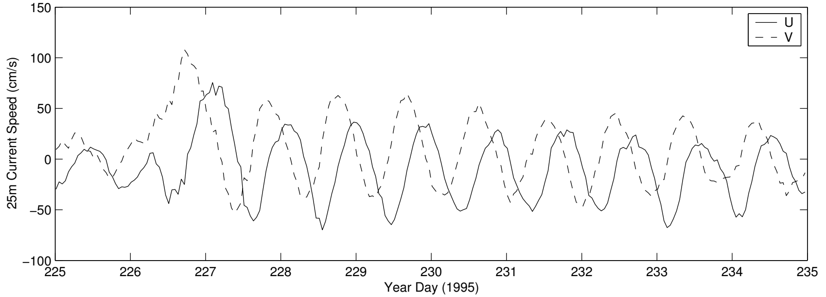
North and East Components of 25m Current Speed After Passage of Hurricane Felix
