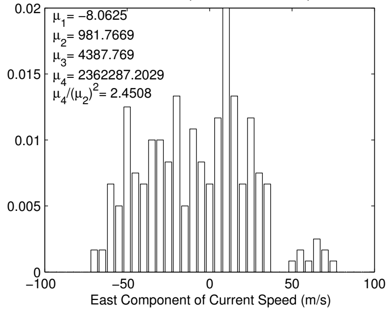
PDF of East Component of Current Speed
