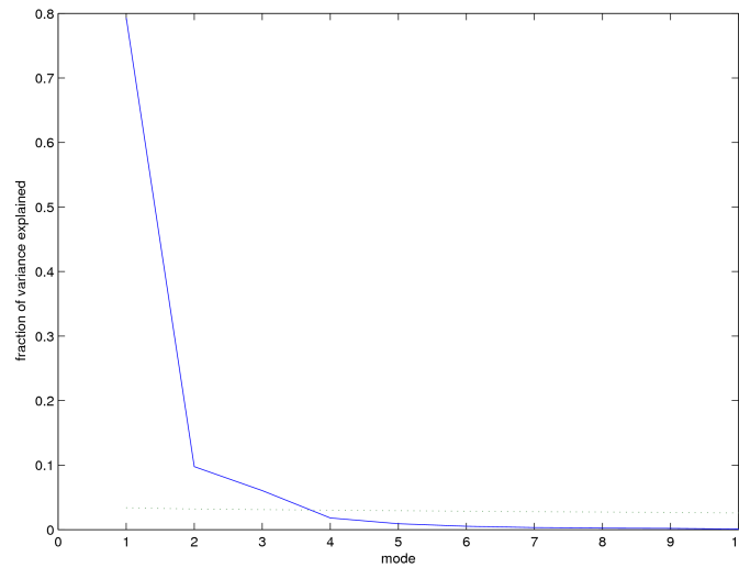
Figure 1: (Solid line) Fraction of variance explained by EOF modes 1 through 10 for Equatorial Pacific temperatures (considered in the MAE 127 notes). Dashed line shows 95th percentile results obtained with random noise.
