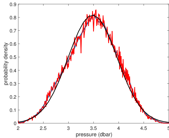
Figure 1: Probability density function for 2017 pressures measured from the shore station at the Scripps pier. Here the blue line indicates the pdf computed using bins with a width of 0.1 dbars, and the red line indicates the pdf for bins with a width of 0.01 dbars. The black line is a Gaussian defined by the mean and standard deviation of the measurements.
