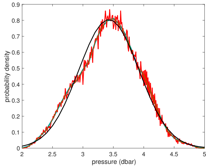
Figure 1: Probability density function for 2018 pressures measured from the shore station at the Scripps pier. Here the blue line indicates the pdf computed using bins with a width of 0.1 dbars, and the red line indicates the pdf for bins with a width of 0.01 dbars. The black line is a Gaussian defined by the mean and standard deviation of the measurements.
