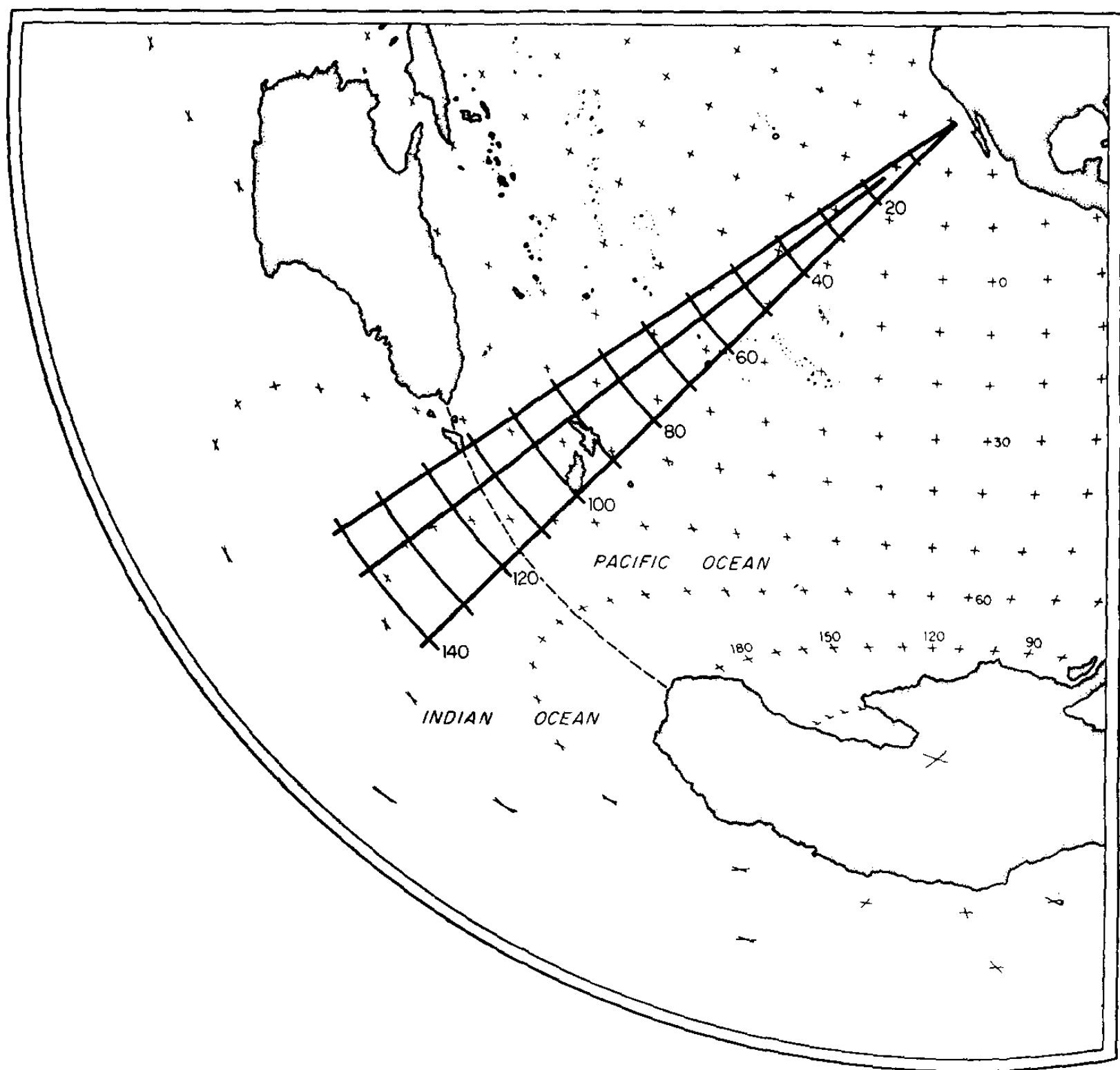
Fig. 6. Azimuthal-equidistant projection centred on San Diego. Distances from Guadalupe are given in units of degrees ( 1^\circ equals 111 km).
