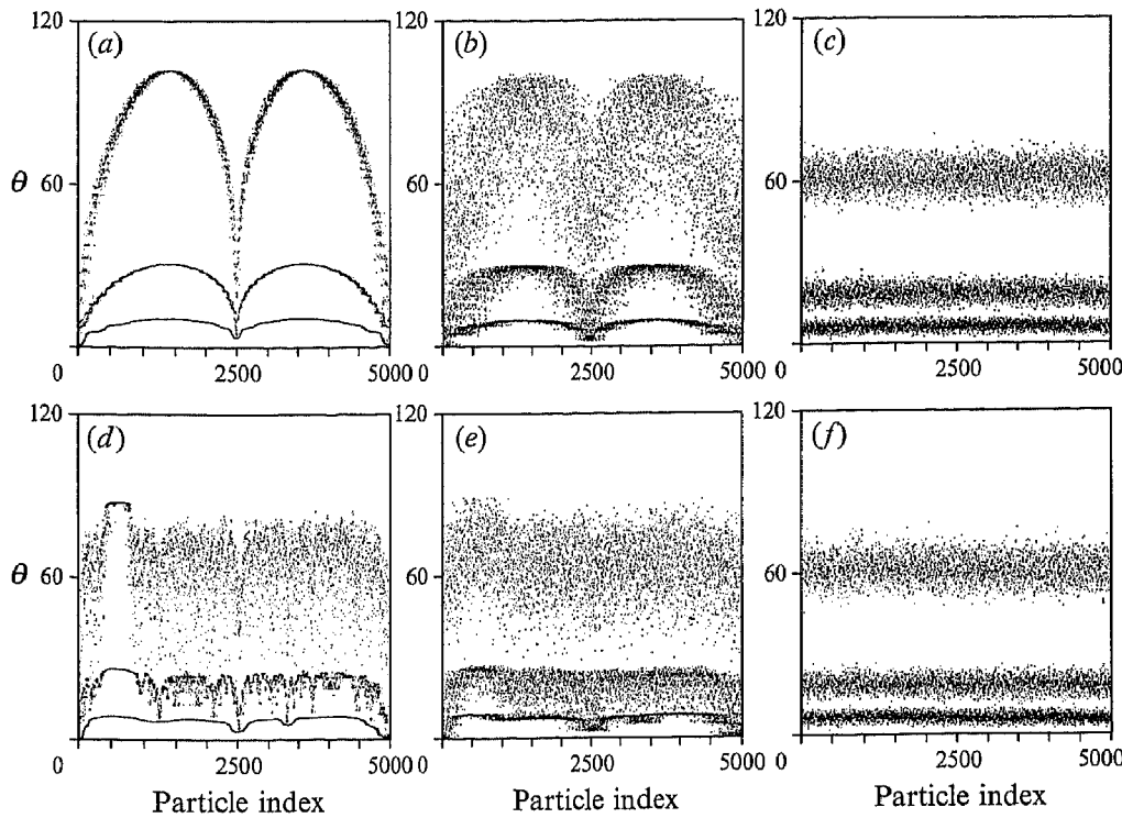
FIGURE 4. Axial dispersion of diffusive particles for the parameter values and times shown in figures 3(a) and (b). The top row shows the dispersion of diffusive tracer in the regular regime. The bottom row shows the dispersion of tracer in the mixed regime. Across each row D is 10^{-6} , 10^{-4} and 10^{-2} . (a)–(c) \chi = 0 ; (d)–(f) \chi = \pi/2 .
