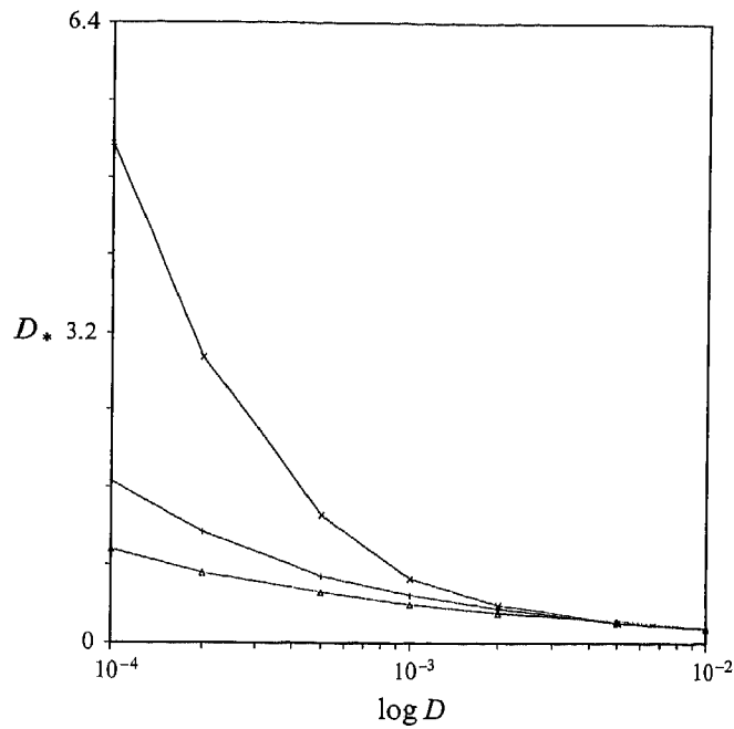
FIGURE 6. The measured value of D_* plotted versus \log D . \times , Re = 25 , \chi = 0 ; + , Re = 25 , \chi = \pi/4 ; \Delta , Re = 25 , \chi = \pi/2 .
