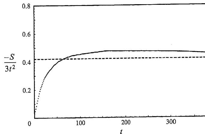
FIGURE 15. A comparison of the analytical result for the unnormalized skewness at long times, given by (4.19) (dashed line), with a twisted-pipe simulation for Re = 62.5 , \chi = \pi/2 .
