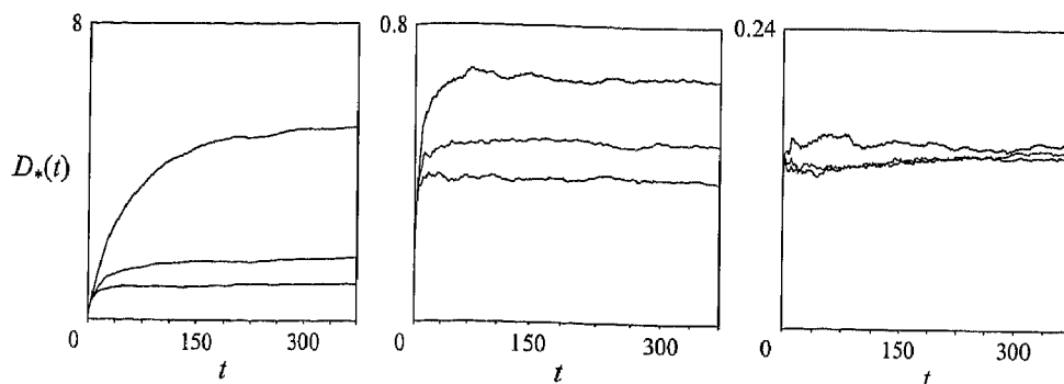
FIGURE 5. The convergence of the function D_*(t) to its asymptotic value for Re = 25 and (a) D = 10^{-4} ; (b) 10^{-3} ; (c) 10^{-2} . In (a) and (b) the upper curve is for \chi = 0 , the middle curve is for \chi = \pi/4 and the lower curve is for \chi = \pi/2 . In (c) the upper curve is for \chi = \pi/2 , the middle curve is for \chi = \pi/4 and the lower curve is for \chi = 0 . Note the change of vertical scale between panels.
