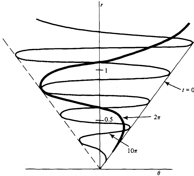
FIGURE 2. The dependence of the advected tracer concentration \theta_A (at \phi = 0 ) on radius for the angular velocity field \Omega(r) = \exp(-r^2) , with \theta(t = 0) = r \cos \phi . The wavelength of the concentration decreases like t^{-1}\Omega_r .
