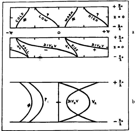
Fig. 1 a. Phase Variations: Above p, \varphi ; Below v_z, \text{div}_H v ; Fig. 1 b. Amplitude Variations: Left p, \varphi ; Right v_z, \text{div}_H v .
